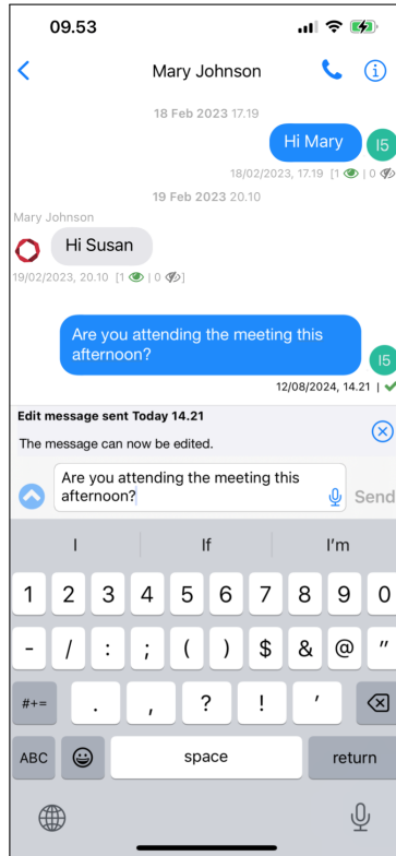
Figure 38: Editing message
