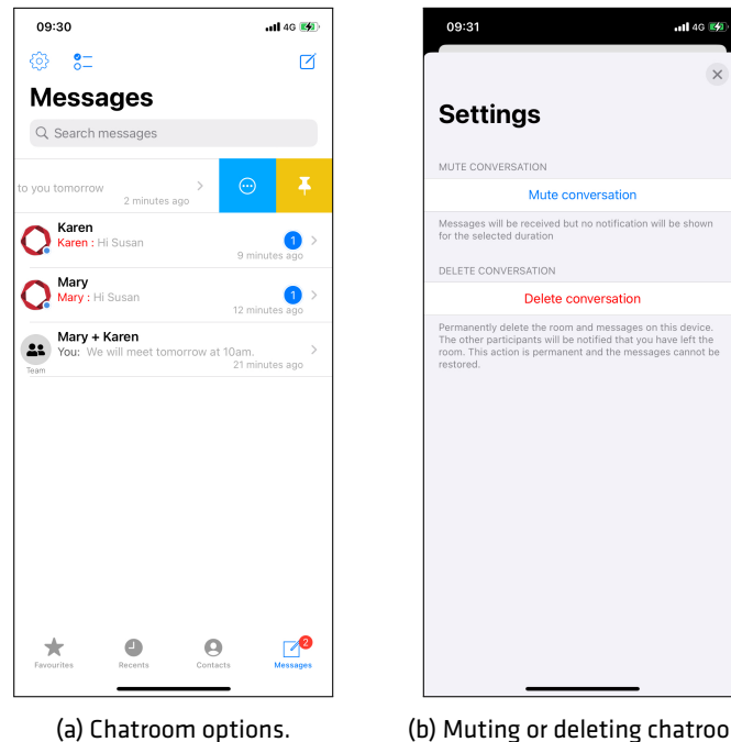
Figure 18: Chatrooms.
