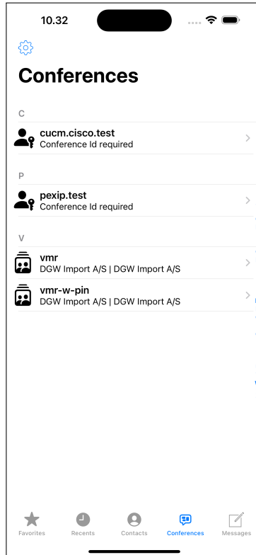
Figure 15: Conferences screen.
