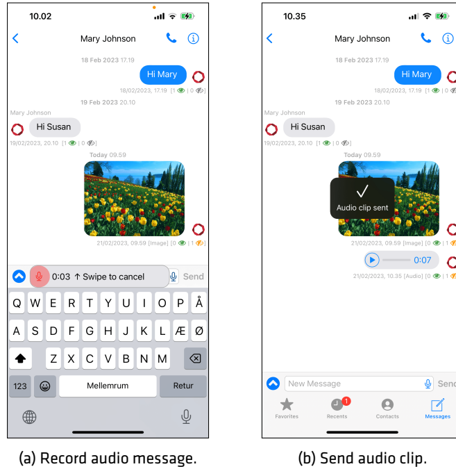
Figure 41: Push-to-Talk messaging
