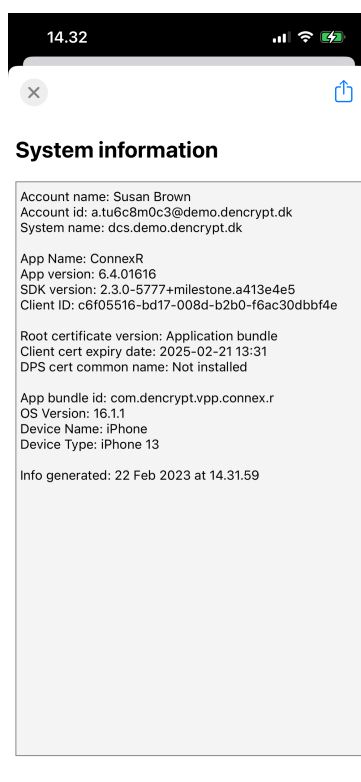
Figure 48: System information
