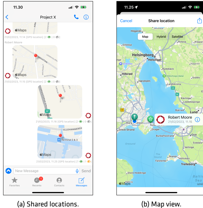
Figure 42: Location sharing
