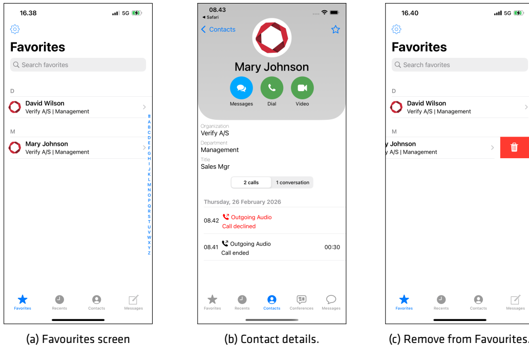
Figure 9: Favourites.
