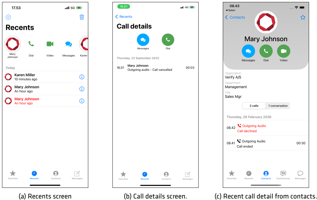
Figure 10: Recents.
